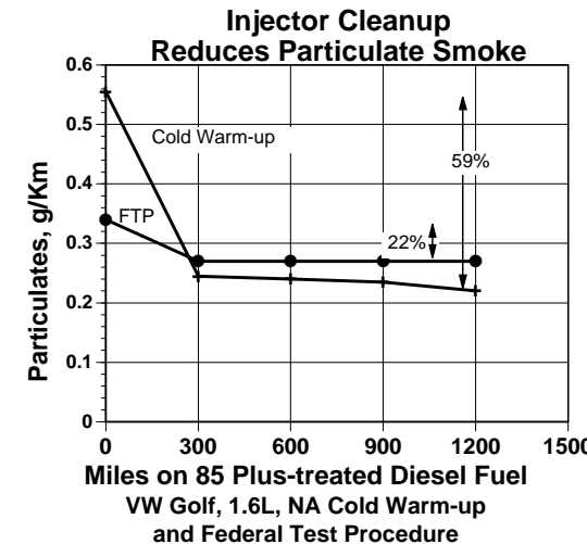
Figure 5: Particulate (smoke) reductions as measured in a Federal Test procedure (warmed-up) and Cold Start/Warm-up Test after 4 ounces 85Plus in 33 gallons.
